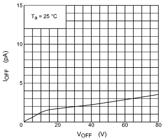
Fig. 12.9 I OFF - V OFF
